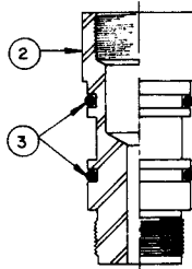
ADAPTER PART NO. 1639
