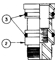
ADAPTER PART NO. 2693
